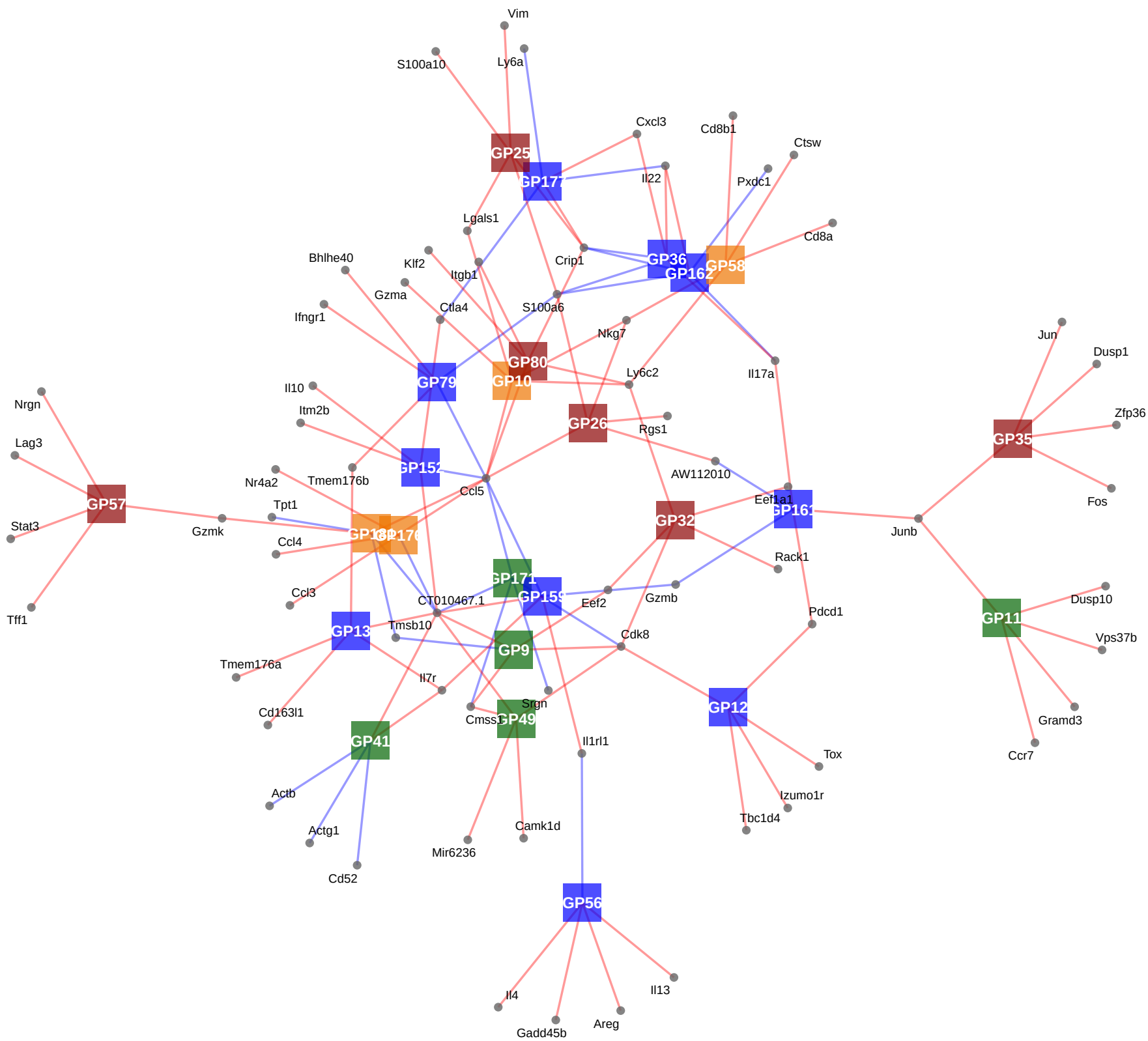
GP-Gene Signature Network Nodes colored by manual GP classification
